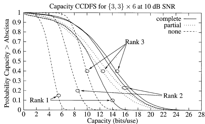
Fig. 6. Capacity CCDFs for different cases of partial channel information.
