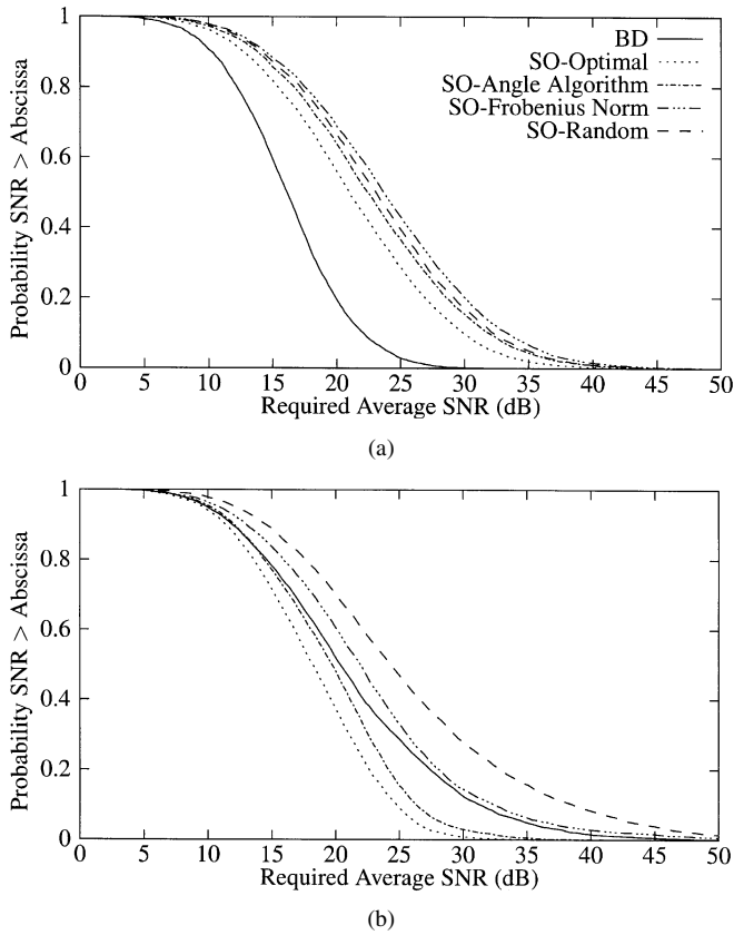
Fig. 7. Performance of successive optimization compared with BD for n_T = 6 , random rate points in the interval [2, 8] , and random channel gains in the interval [-6, 6] dB.
